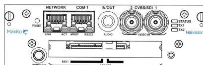
Makito X (Dual SDI) Removable Storage
