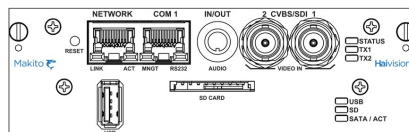
Makito X (Dual SDI) Fixed Storage
